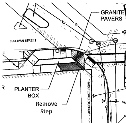
Grade sidewalk to slope as a ramp vs the current step
